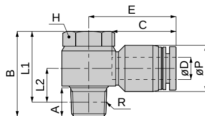
Appearance Dimension for Taper pipe thread (PT)
