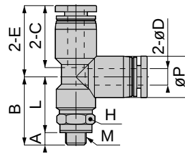
Appearance Dimension for Metric thread
