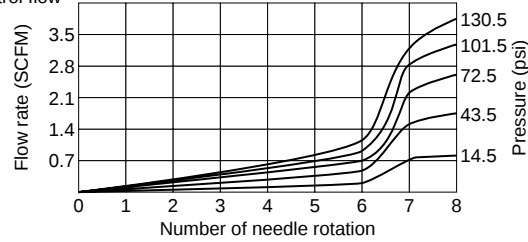
Control flow
