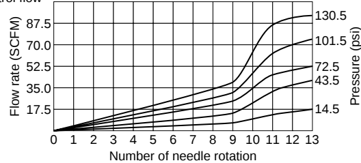
Control flow
