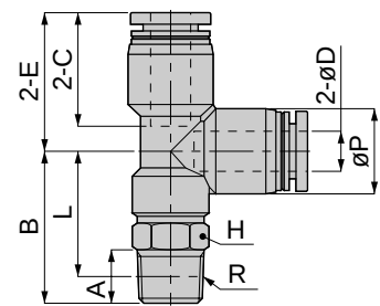
Appearance Dimension for Taper pipe thread (PT)
