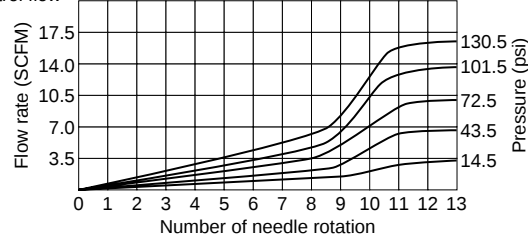
Control flow
